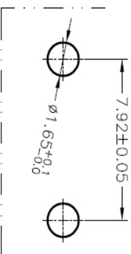
RECOMMENDED HOLE PATTERN
