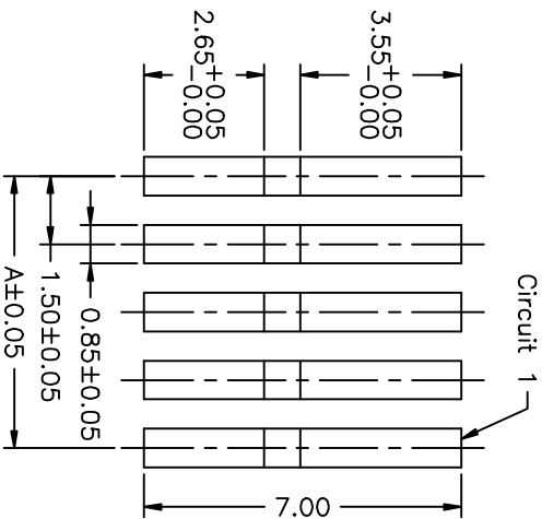
PCB LAYOUT
