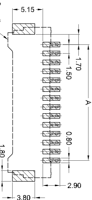
Recommended P.C.B Layout General Tolerance±0.05
