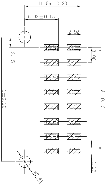
P.C.B Layout: TOP VIEW Tolerance: ±0.05mm
