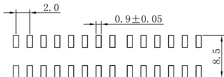
PCB LAYOUT
